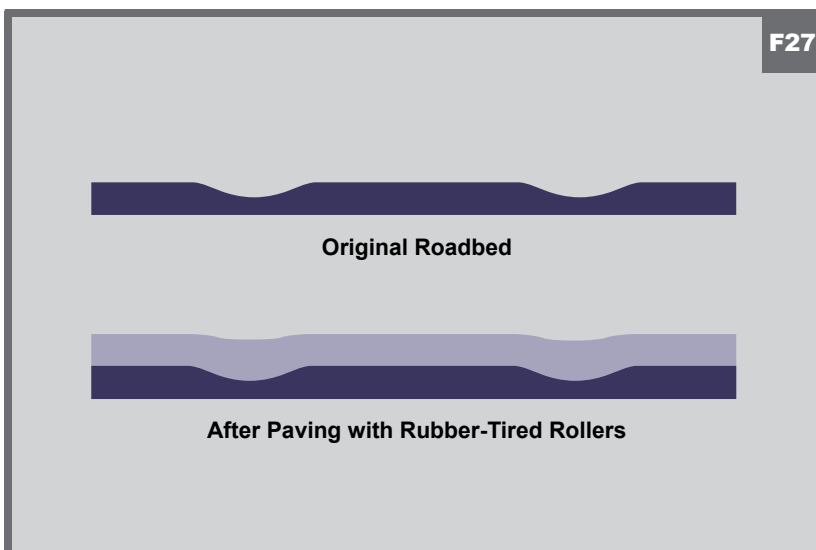
Overlays Can Cause Instant Re-Rutting
