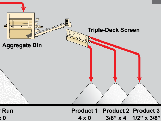
Virgin Aggregate Separated Into Three Sizes
