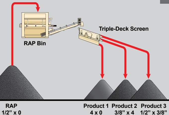
RAP Separated Into Three Sizes
