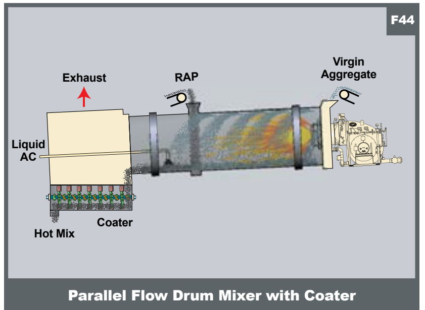
Parallel Flow Drum Mixer
