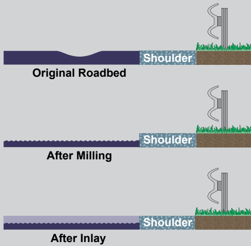
No Shoulder or Guardrail Changes with Milling
