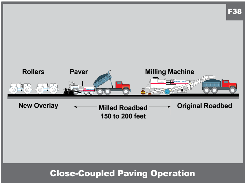
Material Transfer Vehicle and Paver
