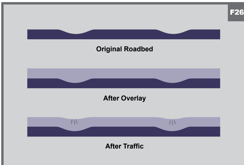
Overlays Can Experience Cracks and Re-Rutting
