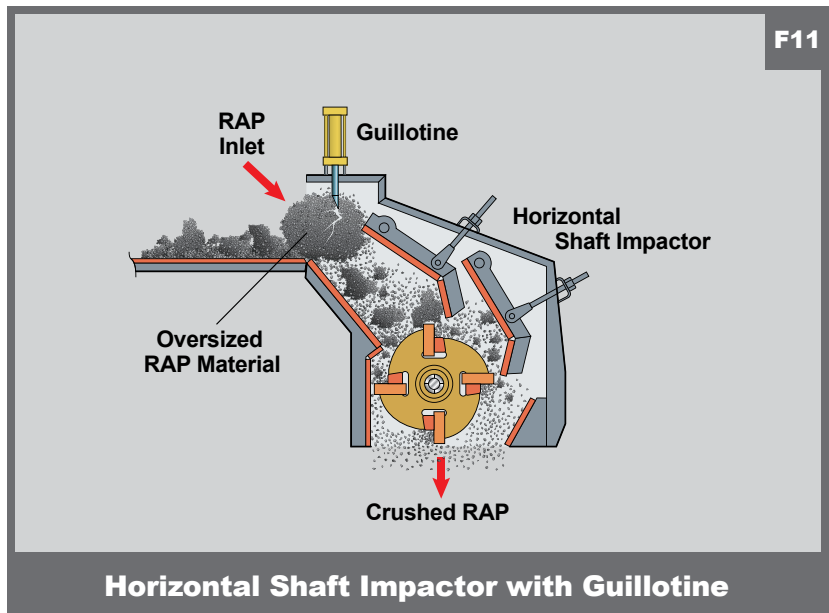
Breaker System
